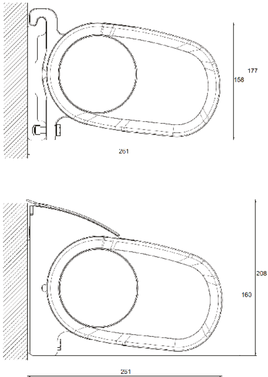
Wall mounting (mm)
